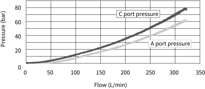
C-A characteristic curves of pressure drop
